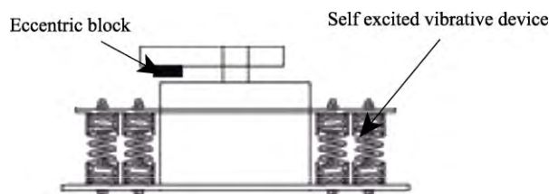
图2 自激振动装置 Fig.2 Self excited vibrative device
