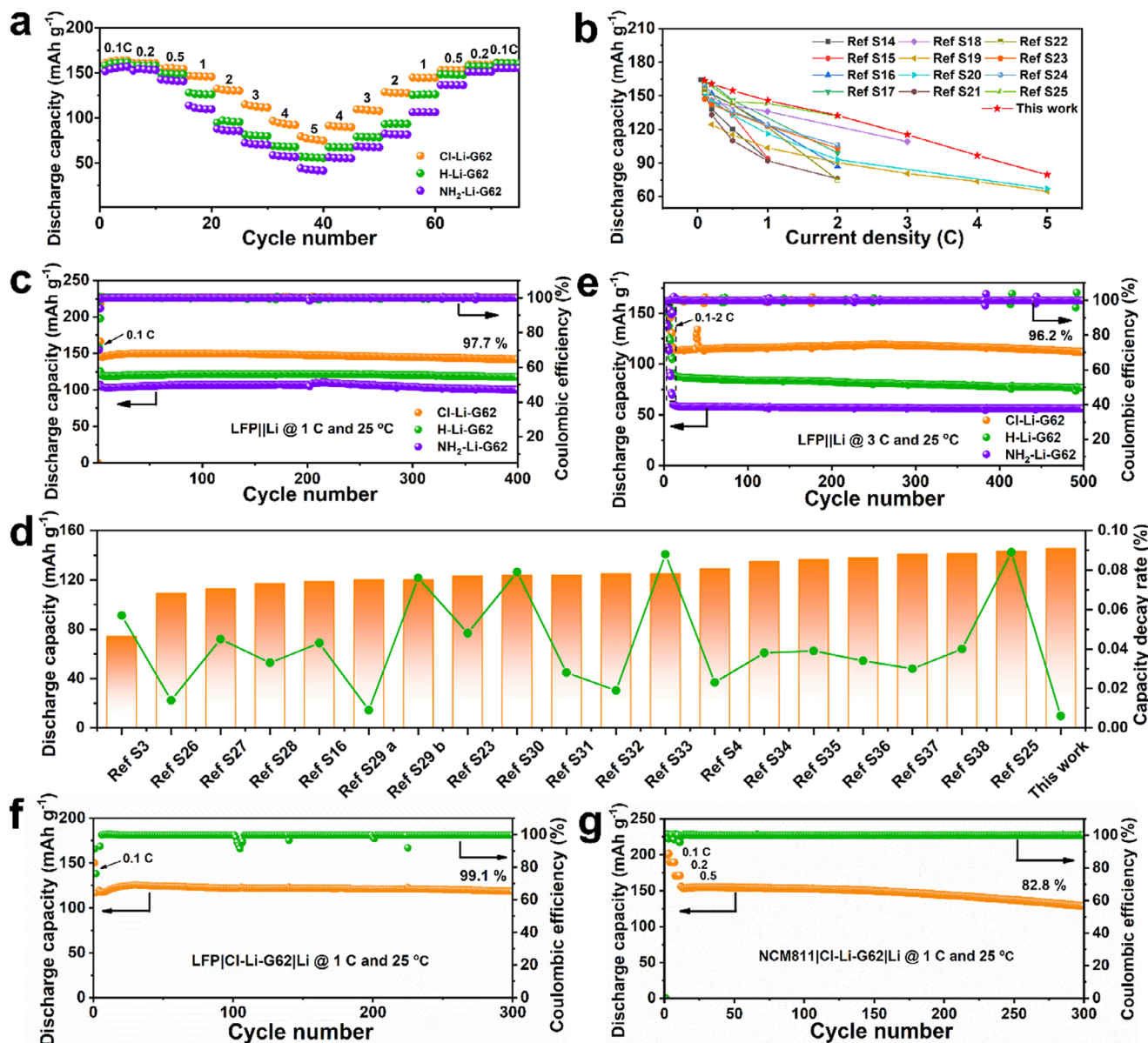
Figure 4. a) Rate performance of LFP|QSSe|Li; b) Rate performance comparisons of Cl-Li-G62 and the reported MOF-based electrolytes; c,e) Cycling stability of LFP|QSSe|Li at 1 and 3C; d) Comparisons of specific capacities at 1C and corresponding average capacity decay rate per cycle of various MOF-based electrolytes; f) Cycling performance of LFP|Cl-Li-G62|Li at 1C after 7-day exposure in air; g) Cyclability of NCM811|Cl-Li-G62|Li at 1C.
